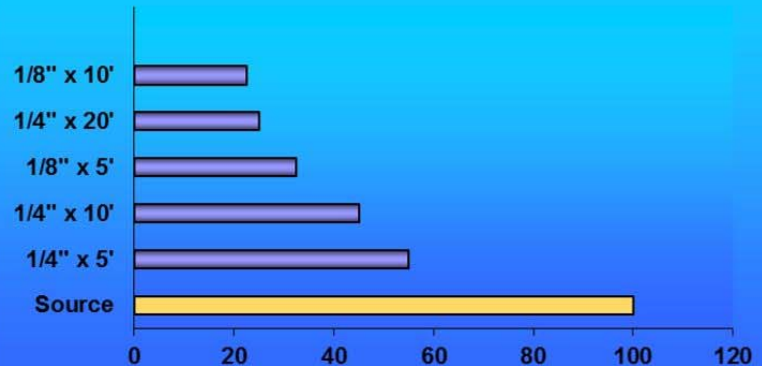
% Light Transmission
